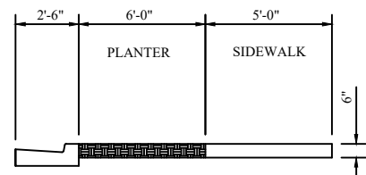
55'-0" RIGHT-OF-WAY
