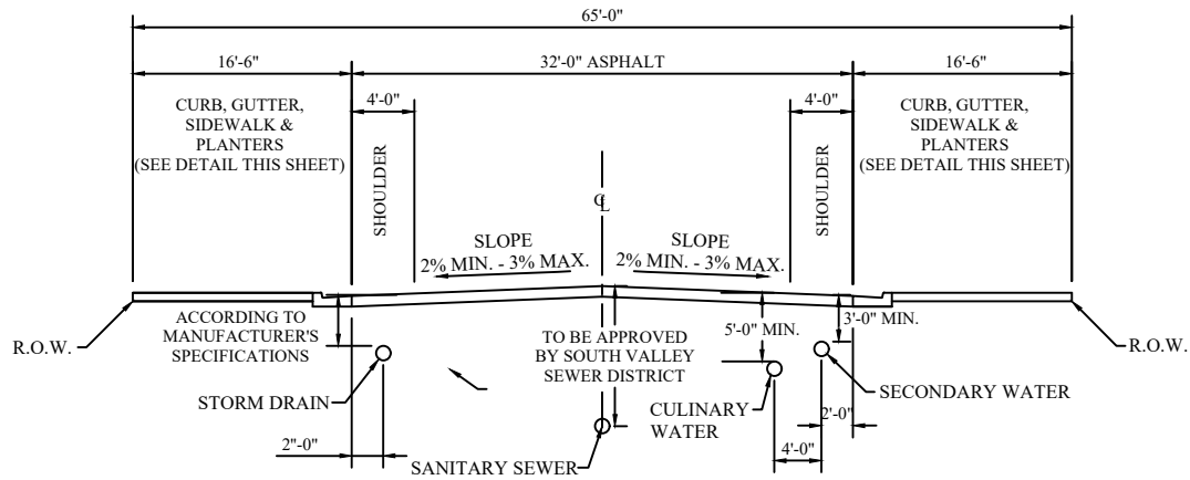
MAJOR LOCAL - 65'-0" RIGHT-OF-WAY
