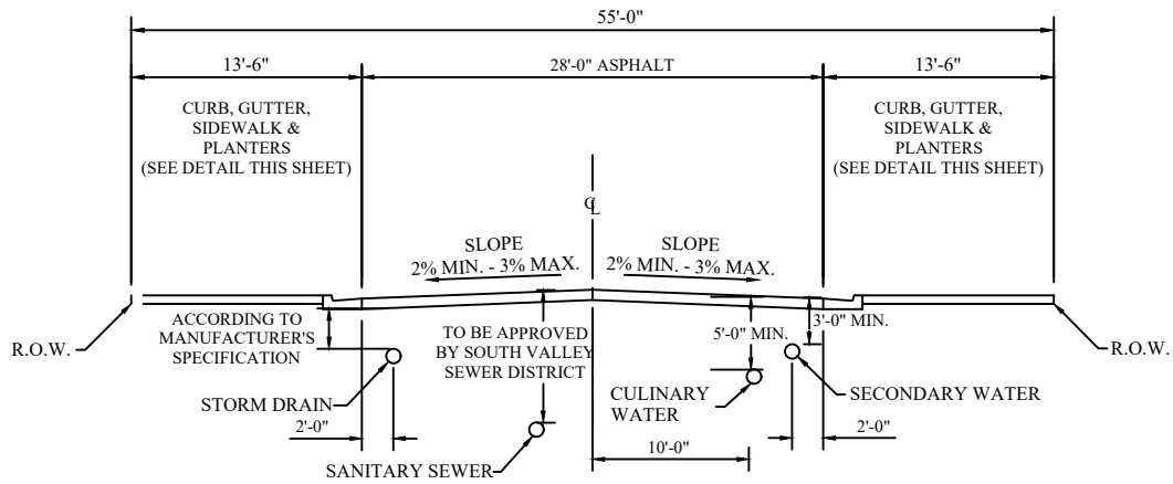
MINOR LOCAL - 55'-0" RIGHT-OF-WAY
