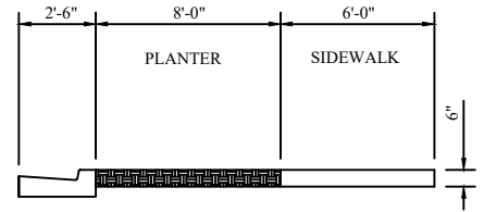
65'-0" RIGHT-OF-WAY
