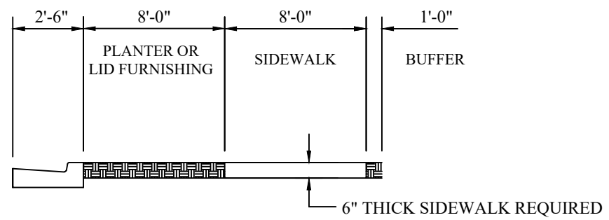
120'-0" RIGHT-OF-WAY
