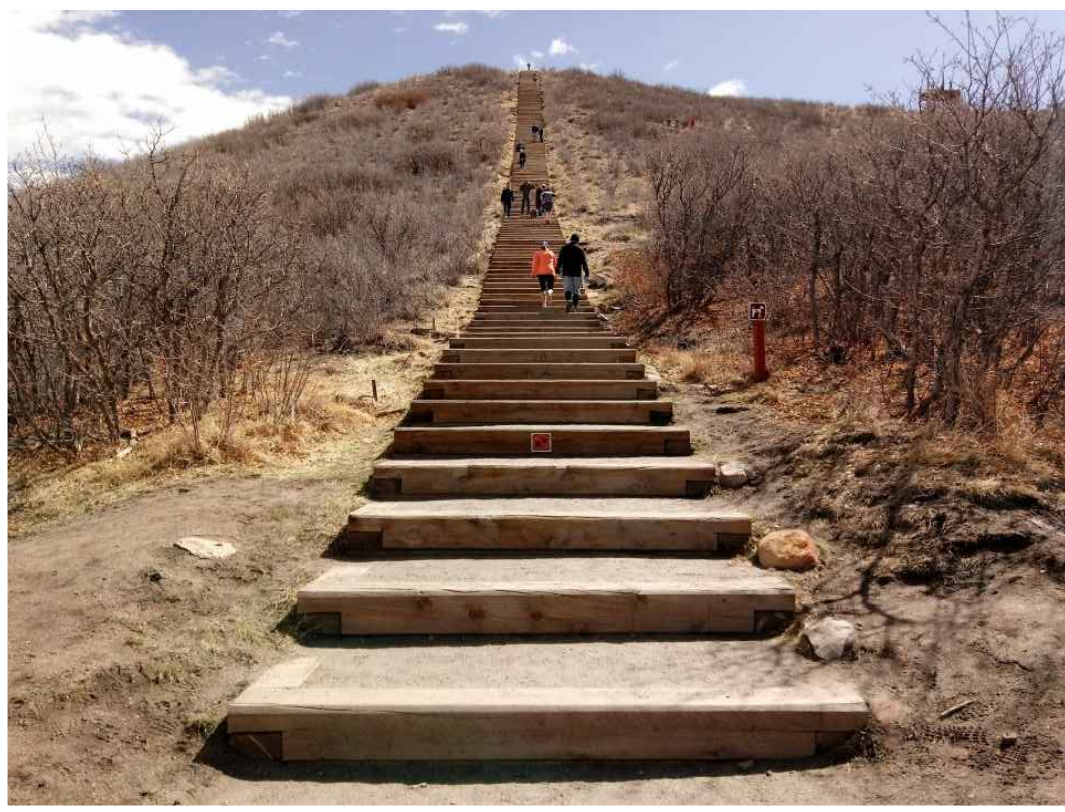
TIMBER STAIR RISERS WITH CRUSHED STONE
