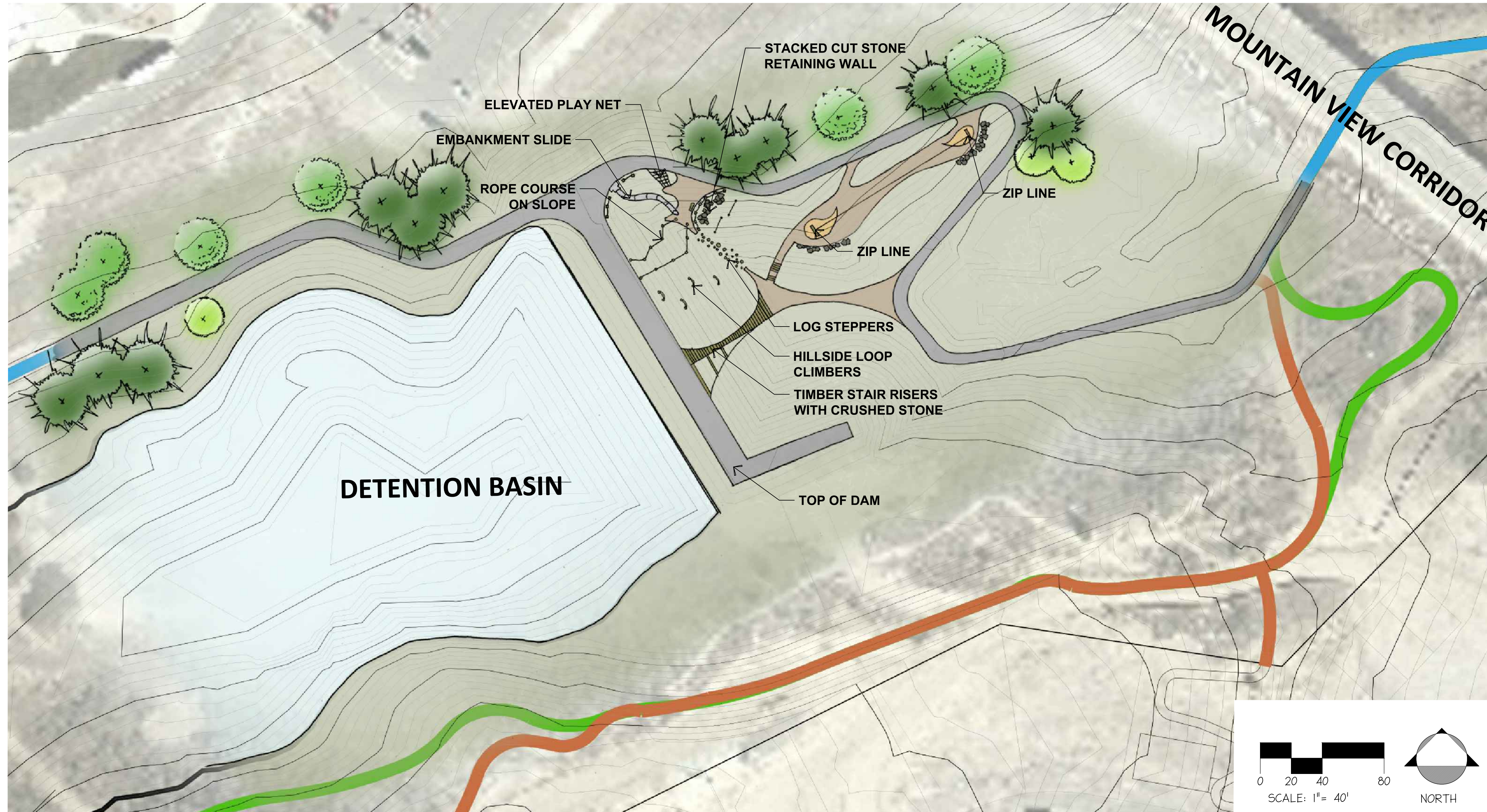
EMBANKMENT SLIDE
